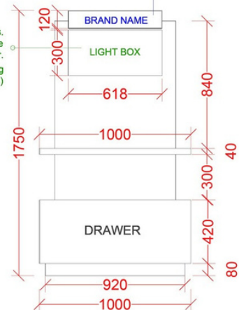
DISPLAY STAND / A TOP BOX The upper box will be illuminated. Top box is available on both surfaces.
